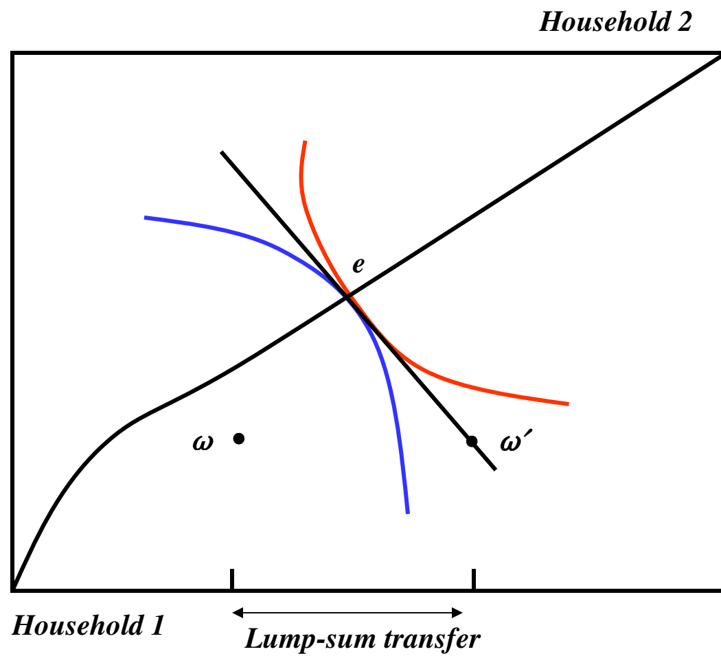
Figure 2: Second Welfare Theorem
